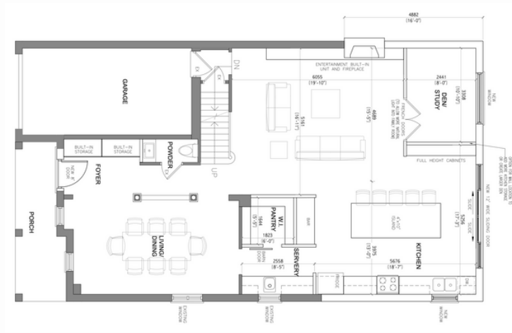
Floor plans
